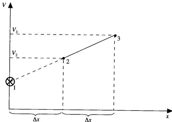
FIG. 7.7 Sketch for linear extrapolation.
