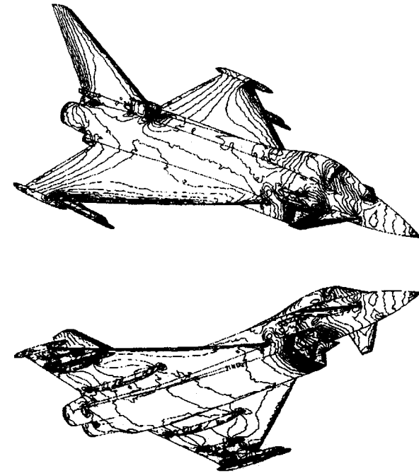
FIG. 6.34 Three-dimensional pressure coefficient contours over the surface of a generic fighter aircraft. M_\infty = 0.85 , angle of attack = 10^\circ , angle of yaw = 30^\circ . (From Ref. 73. Courtesy of Elsevier Science Publishers.)
