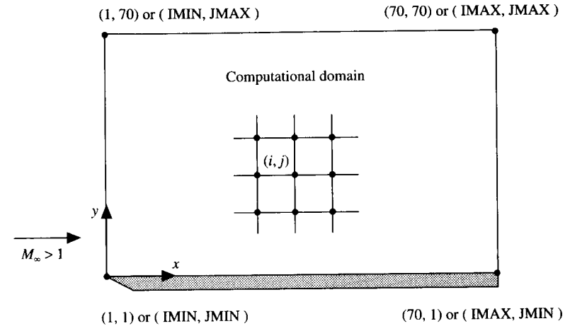
FIG. 10.3 Computational domain.
