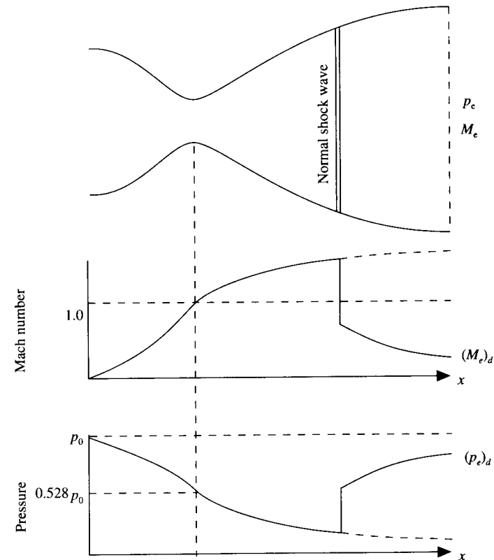
FIG. 7.21 Schematic of a nozzle flow with an internal normal shock wave.
