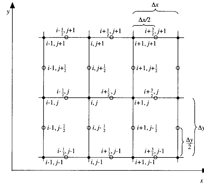
FIG. 6.15 Staggered grid.
